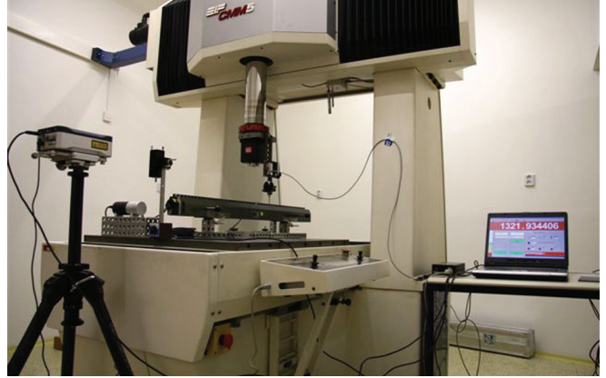
CMI Laboratory of Technical Length: Touch-probe CMM5-SIP.
