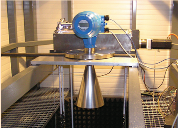
Radar level gauge being calibrated in the Laboratory of Flow and Heat.
